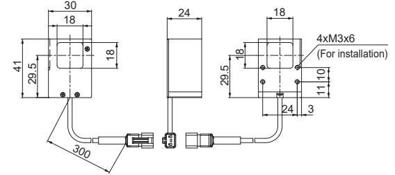
LFV3-CP18IR2-860/950
