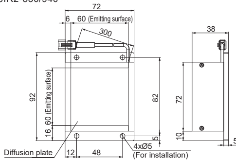
LDL-60X60IR2-850/940
