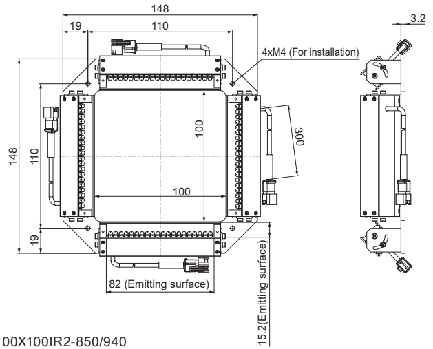
LDL-100X100IR2-850/940
