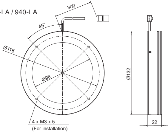
LDL-42X15IR2-850/940
