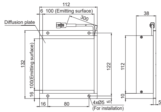
LDL-100X100IR2-850/940
