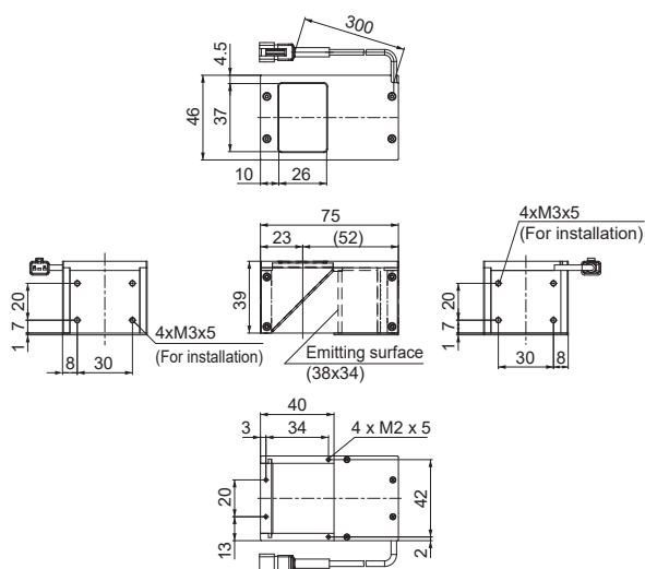
LFV3-35IR2-850(A)/940(A)
