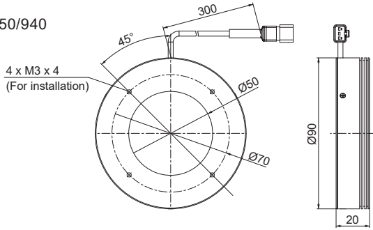
LDR2-74IR2-850-LA / 940-LA
