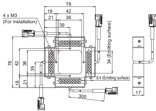
LDQ-78IR2-850/940
