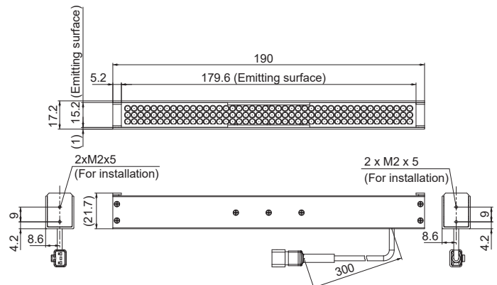
LDL-180X15IR2-850/940
