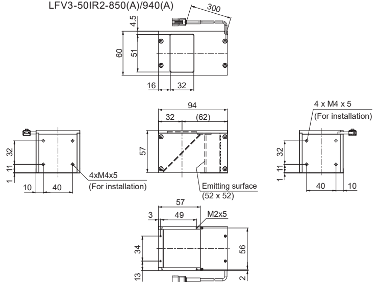
LFV3-50IR2-850(A)/940(A)
