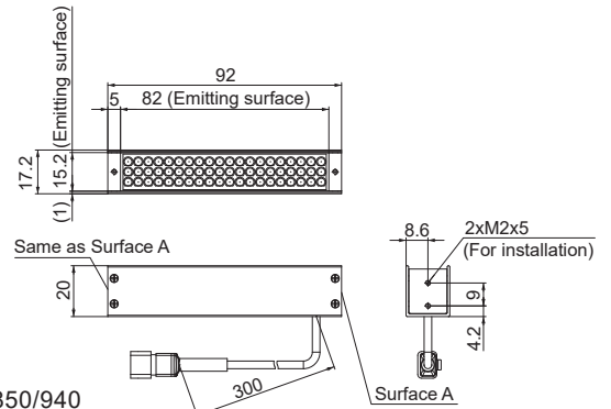
LDL-82X15IR2-850/940
