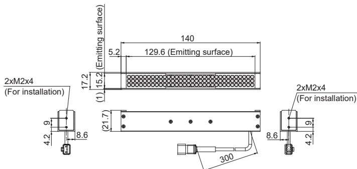
LDL-130X15IR2-850/940
